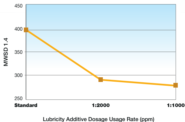
AR6400-D MAX - Friction Test Results
